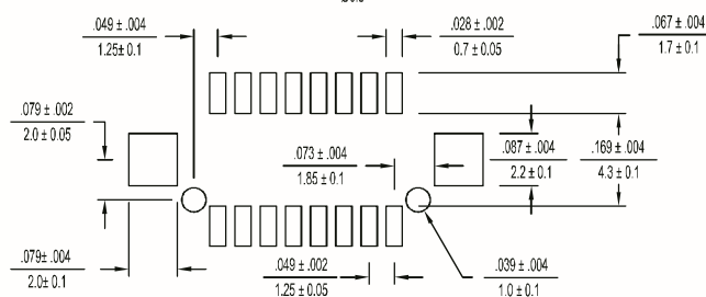
PCB Layout: Solder side
