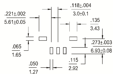
PCB Layout: Component side
