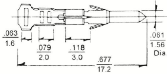
Tin Plated Brass Terminal
